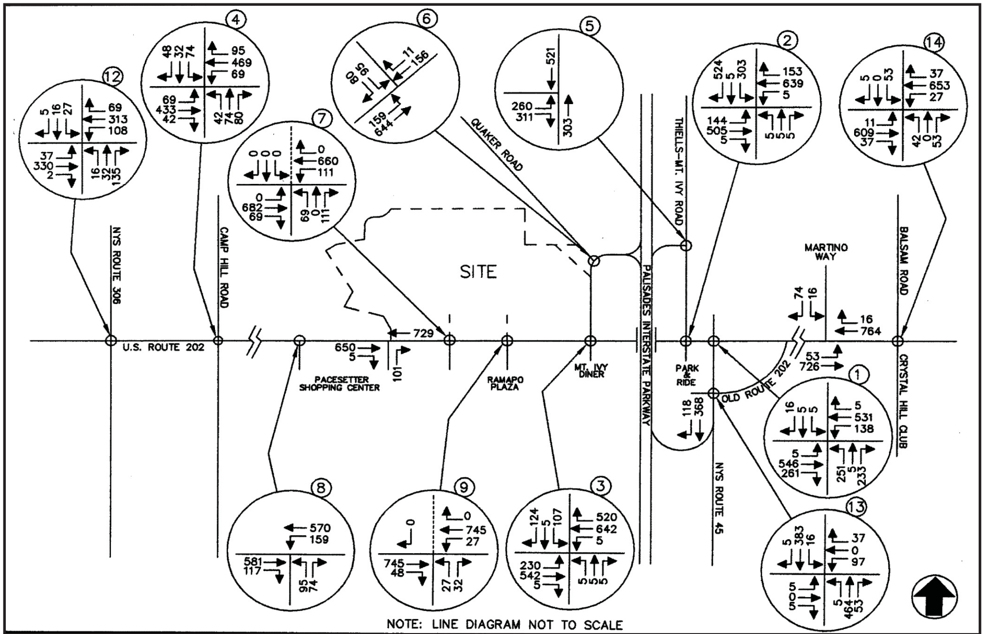
Figure 3.5-32: 2011 No-Build Traffic Volumes Weekend Peak Saturday Highway Hour (With Patrick Farm) Minisceongo Park Towns of Haverstraw & Ramapo, Rockland County, New York Source: John Collins Engineers, P.C. Date: October, 2008
